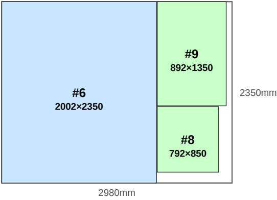
Segment #4 - Length: 2350mm (Scale: 50mm = 1mm)
